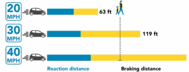
Figure 3.18 Perception-Reaction Time
